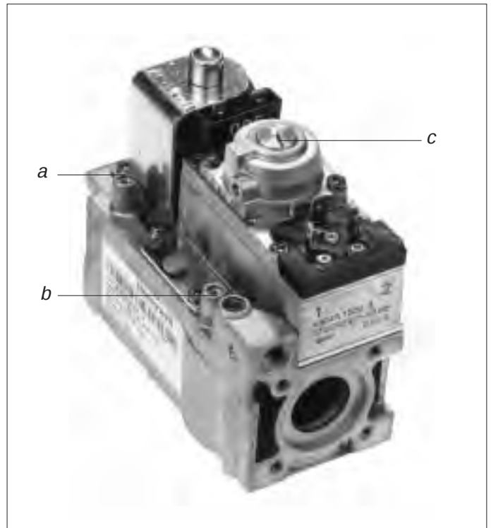
Afb. 12 Honeywell VR 4601 CB 1024B (2 per ketel)
